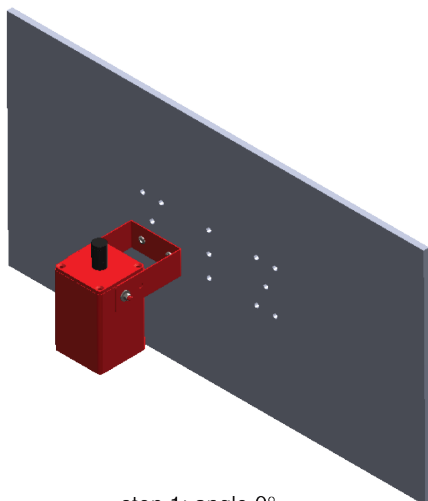
step 1: angle 0°
